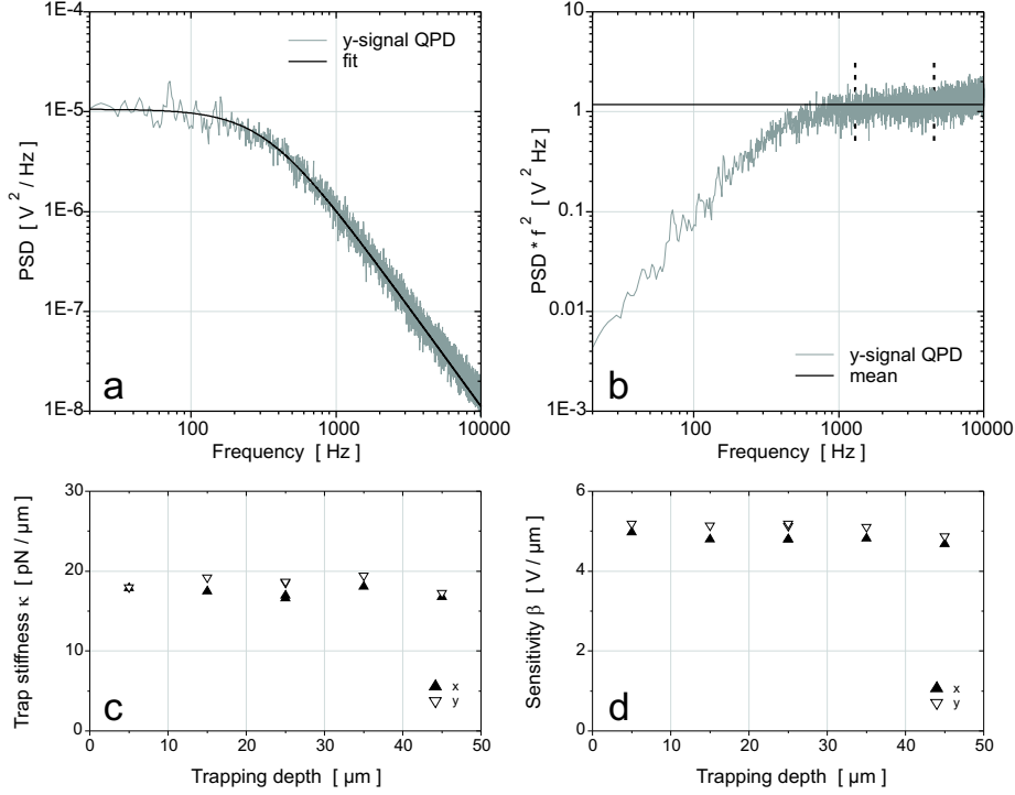
Fig. 7.3: Data for a 1.0\text{-}\mu\text{m} -diameter silica particle in water, trapped in inverted tweezers using a water immersion objective. (a) Power spectral density (PSD) for 420\text{ mW} at the back focal plane, and a Lorentzian fit to the curve with f_0 = 325\text{ Hz} . (b) \text{PSD} \times f^2 curve, with plateau value P_V = 1.18\text{ V}^2 \text{Hz} , the mean of the plateau between the two dashed lines. (c) Trap stiffness \kappa and (d) the sensitivity obtained from the plateau value P_V , for the particle trapped at different depths in the 50\text{-}\mu\text{m} -thick sample. (a) and (b) are the data for the y -signal at 15\text{ }\mu\text{m} into the sample.
