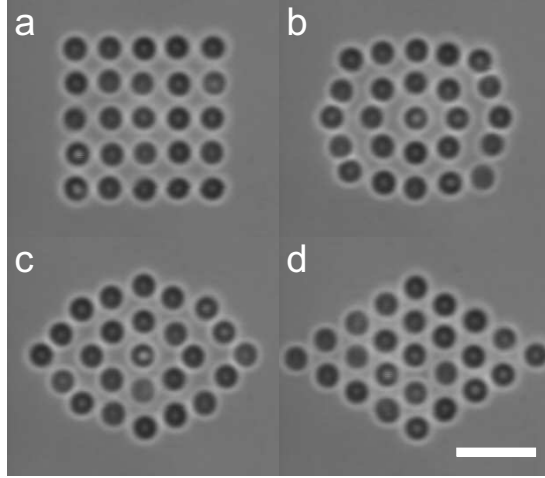
Fig. 2.4: (a) Transmission microscopy image of 1.4- \mu m-diameter FITC-SiO 2 particles trapped in an array of 25 time-shared optical traps with squared symmetry. The inverted objective was used for trapping as well as for imaging. Using the AODs, the pattern was dynamically changed in a few seconds without losing particles, via intermediate patterns (b) and (c) to an array with triangular symmetry (d). The scale bar is 5 \mu m.
