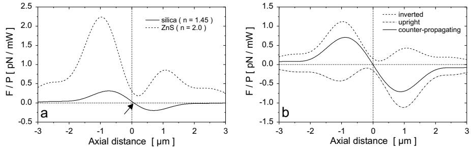
Fig. 1.2: Force per Watt laser power along the beam axis. (a) Curves for a silica particle ( n = 1.45 ) and a ZnS ( n = 2.0 ) particle, both 1\ \mu\text{m} in diameter, trapped in water ( n = 1.33 ) in a single-beam trap. The silica particle is trapped close to the laser focus, but the ZnS particle has no stable trapping position. (b) Curve for a 1\text{-}\mu\text{m} -diameter ZnS particle trapped in counter-propagating traps (solid line). The particle is trapped at the overlapping foci of the beams ( z = 0 ). The individual two beams coming from either side (with half the laser power each) are also shown.
