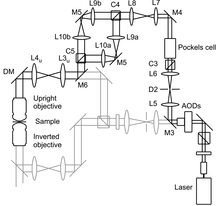
Fig. 2.2: Setup for the creation of arrays of tweezers in two trapping planes. A Pockels cell and beam splitting cubes ( C4 and C5 ) were used to switch between the planes. The Pockels cell and the AODs were synchronized to create independent configurations of traps in each plane. The upright objective was used for trapping, while the inverted objective was used for imaging. The part of the setup drawn in light gray was not used when two trapping planes were created.
