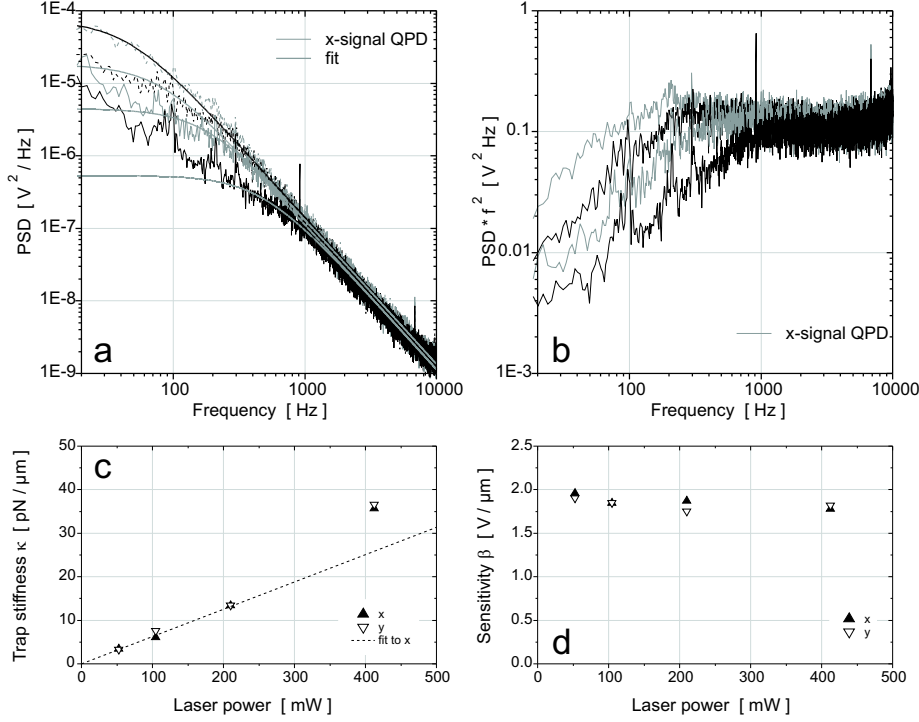
Fig. 7.6: (a) Power spectral density (PSD) curves for a 1.3\text{-}\mu\text{m} -diameter \text{TiO}_2 particle trapped in water using counter-propagating tweezers. The sums of the laser powers at the back focal planes of the two objectives were 52, 105, 210, and 412 mW. The highest power yields the lowest plateau value. (b) The corresponding \text{PSD} \times f^2 curves. (c) Trap stiffness \kappa and (d) the sensitivity obtained from the plateau value P_V , for the four powers. In (c) the fit to the first three data points for x is shown ( \kappa = 62.6 \text{ pN}/\mu\text{m}/\text{W} ).
