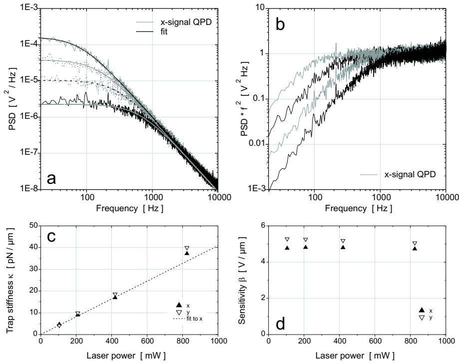
Fig. 7.5: Data for a 1.0\text{-}\mu\text{m} -diameter silica particle in water, trapped in inverted tweezers using a water immersion objective. (a) Power spectral density (PSD) curves for the x -signal, for 105, 210, 420, and 825 mW at the back focal plane, and Lorentzian fits to the curves with f_0 = 79, 151, 286 , and 628 Hz, respectively. (b) The corresponding \text{PSD} \times f^2 curves. (c) Trap stiffness \kappa and (d) the sensitivity obtained from the plateau value P_V , for the four powers. In (c) the fit to the first three data points for x is shown ( \kappa = 40.9 \text{ pN}/\mu\text{m}/\text{W} ).
