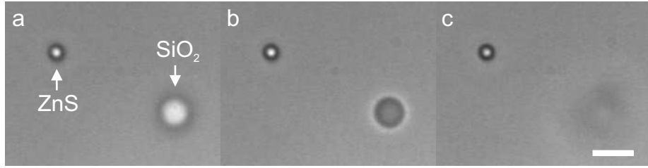
Fig. 2.8: A 0.5\text{-}\mu\text{m} -diameter ZnS particle (left) trapped in counter-propagating optical tweezers next to a 1.4\text{-}\mu\text{m} -diameter FITC-SiO 2 particle (right) that was stuck to the surface of the sample cell. The ZnS particle was trapped in three dimensions, as can be seen in (b) and (c), where the sample was moved down with respect to the trapping plane; the ZnS particle was trapped and therefore stayed in focus, while the FITC-SiO 2 particle moved out of the focal plane. It was not possible to trap the ZnS particle using single-beam optical tweezers. The scale bar is 2\text{ }\mu\text{m} .
